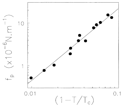
FIG. 4. Pinning force at one particular site in the Pb film plotted as a function of (1 - T/T_c) . The straight line is a fit to an empirical form (see text).
