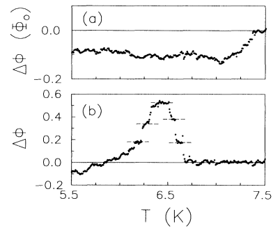
FIG. 2. (a) The change in flux ( \Delta\phi ) threading a Hall probe as a function of temperature at an applied field of 0.5 mT. (b) The same measurement at an applied field of 10 mT.
