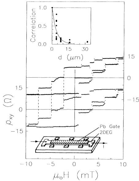
FIG. 1. Hall resistivity measured simultaneously at two Pb-gated detectors with 4 \mu\text{m} separation at 4.3 K. A resistivity of 1 \Omega corresponds to a single flux line threading the 2 \mu\text{m} \times 2 \mu\text{m} detector. The lower inset shows a sketch of the sample. The upper inset plots the correlation coefficient at various contact separations.
