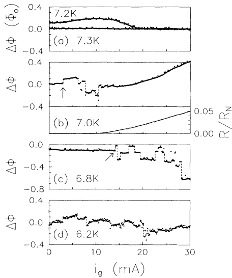
FIG. 3. (a)–(c) The change in flux ( \Delta\phi ) threading a Hall probe as a function of gate current I_g in an applied field of 1 mT at various temperatures and (d) in 10 mT at 6.2 K. The arrows indicate the feature used to build Fig. 4. Included in (b) is the I - R curve of the Pb gate normalized by the resistance at 8 K.
