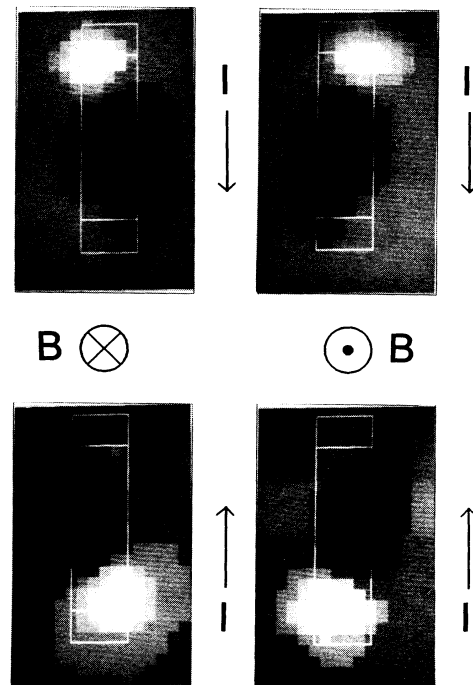
FIG. 3. Photoconductivity images of the two-terminal resistance corresponding to the four possible permutations of magnetic field and current direction. The dark areas correspond to an increase in the resistance.
