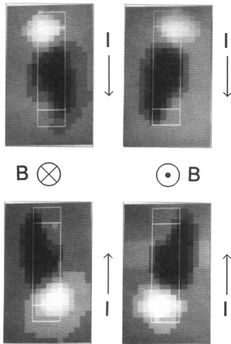
FIG. 3. Photoconductivity images of the two-terminal resistance corresponding to the four possible permutations of magnetic field and current direction. The dark areas correspond to an increase in the resistance.
