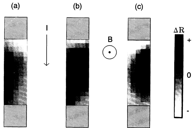
FIG. 4. Images of the change in two-terminal resistance at three different filling factors. (a) E_F just below an empty Landau level, (b) E_F midway between two levels, and (c) E_F just above a filled level.
