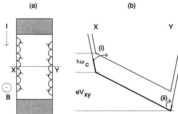
FIG. 1. (a) Skipping orbits of electrons at edges of 2DEG in a strong magnetic field. (b) Schematic diagram of electronic energy levels on a line X-Y through the center of the device assuming a uniform distribution of Hall field across the sample width.
