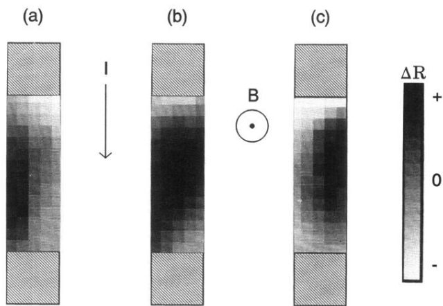
FIG. 4. Images of the change in two-terminal resistance at three different filling factors. (a) E_F just below an empty Landau level, (b) E_F midway between two levels, and (c) E_F just above a filled level.
