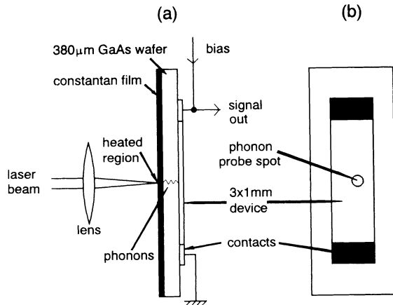
FIG. 2. Sample geometry: (a) Side view, the laser beam is positioned on the Constantan film using a pair of galvanometer driven x - y mirrors under computer control. (b) Top view (sample face), the light-shaded area indicates the approximate size of the phonon probe beam.
