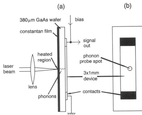
FIG. 2. Sample geometry: (a) Side view, the laser beam is positioned on the Constantan film using a pair of galvanometer driven x - y mirrors under computer control. (b) Top view (sample face), the light-shaded area indicates the approximate size of the phonon probe beam.
