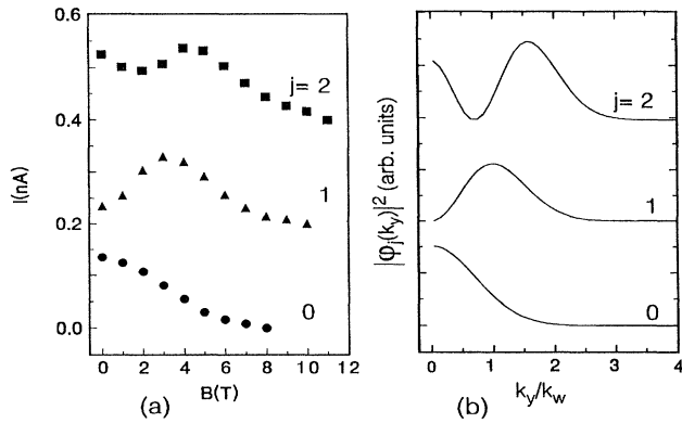
FIG. 3. (a) Variation of peak currents with magnetic field for the j = 0, 1 , and 2 (circles, triangles, and squares, respectively) peaks. The experimental data are displaced for clarity. (b) |\Phi_j(k_y)|^2 the probability densities for the j = 0, 1 , and 2 simple harmonic oscillator states. k_w = [(m\omega_w/\hbar)^{1/2}] is the natural wave vector for a SHO state. The maximum for the j = 1 state occurs at k_y/k_w \approx 1 and experimentally at B \approx 3.1 T corresponding to a value of k_0 = eB\Delta s/\hbar \approx 9.1 \times 10^7 \text{ m}^{-1} . Equating this value with k_w gives \hbar\omega_w = 10 meV.
