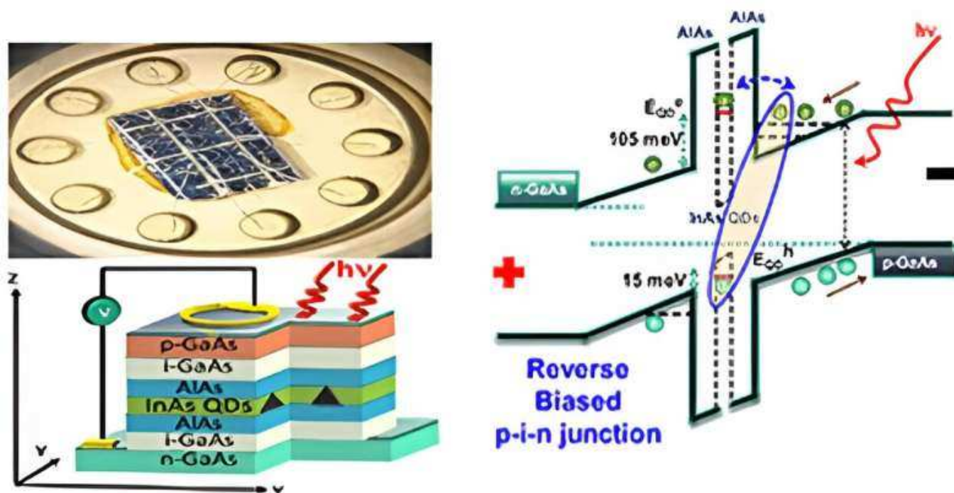
Figure. 1. A schematic diagram of GaAs/AlAs/InAs/AlAs/GaAs double-barrier, 0D-2D heterostructure. Corresponding energy band-diagram is shown on the right. Oval shape shows the formation of 0D-2D indirect exciton. Credit: Materials Today Electronics (2023). DOI: 10.1016/j.mtelec.2023.100039
