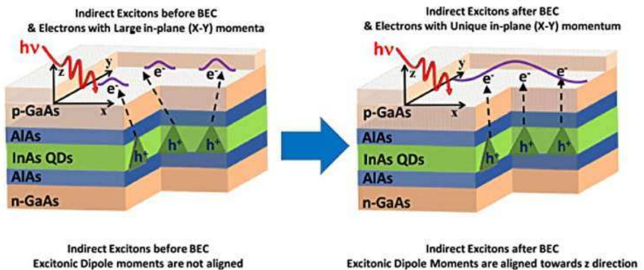
Figure 2. Schematics of spontaneous enhancement of electric polarization of 0D-2D excitons before and after excitonic dipoles collectively align along the vertical z direction during BEC. The small purple contours on the left represent the wave functions of individual excitons before the onset of BEC. The large wave function on the right roughly represents the macroscopic quantum state of excitonic BEC. Credit: Materials Today Electronics (2023). DOI: 10.1016/j.mtelec.2023.100039
