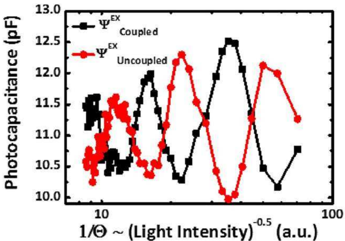
Figure 3. Rabi oscillations of two-level "macroscopic" quantum states of coupled and uncoupled excitons at 10.5 K
